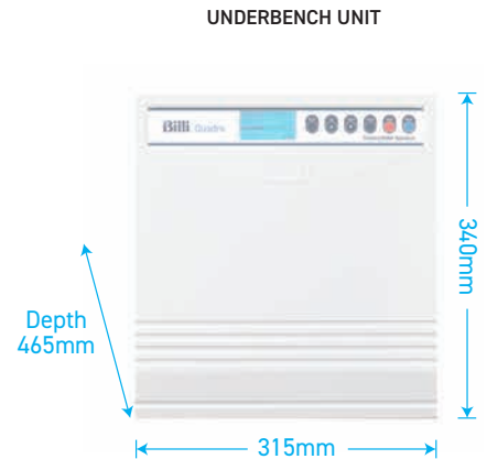
UNDERBENCH UNIT
